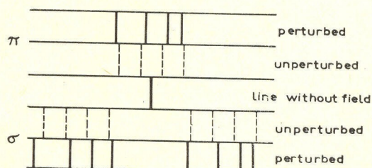
FIGURE 1. Comparison of positions of components in a perturbed and an unperturbed pattern. In a perturbed pattern either the \pi - or the \sigma -components are unequally spaced, in contrast to the unperturbed pattern.
