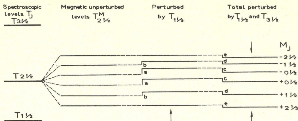
FIGURE 3. Perturbation of magnetic levels of T_{2\frac{1}{2}} due to the proximity of the magnetic levels of T_{1\frac{1}{2}} and T_{3\frac{1}{2}} .
