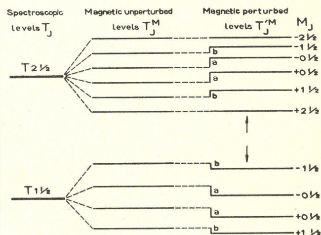
FIGURE 2. Mutual repulsions between the magnetic levels of T_{2\frac{1}{2}} and T_{1\frac{1}{2}} .
